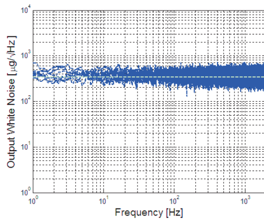
Figure 31: Typical white noise
