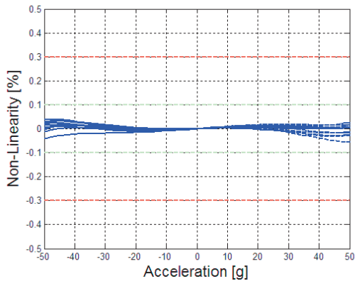
Figure 24 : Non linearity under vibration
