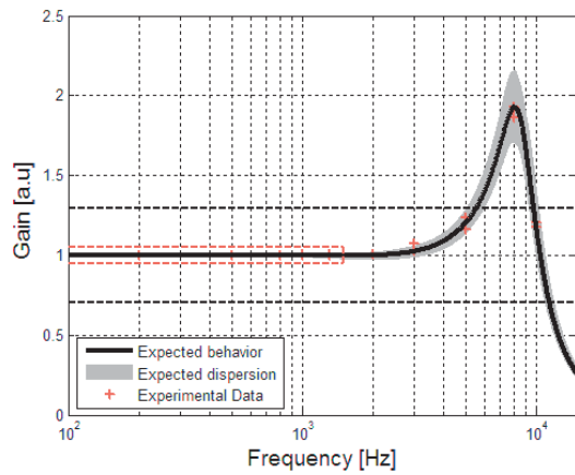
Figure 28: Typical high frequency response Courtesy of Customer
