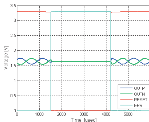
Figure 40: Typical sensor reset sequence with external reset
