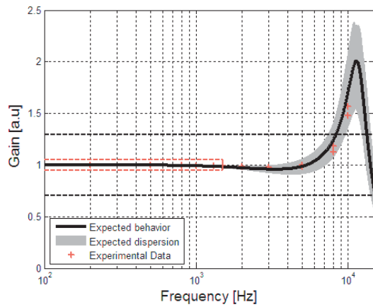
Figure 33: Typical high frequency response Courtesy of Customer
