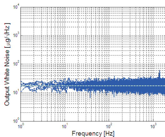
Figure 11: Typical white noise
