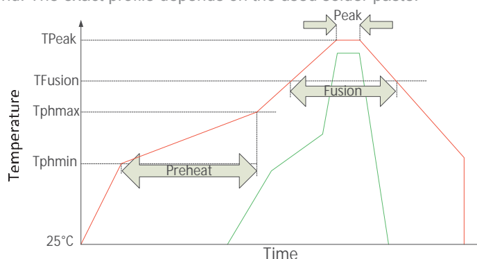
Figure 46: Soldering Temperature Profile
