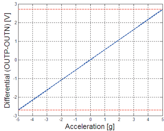
Figure 10: Differential acceleration output (OUTP-OUTN) at full scale
