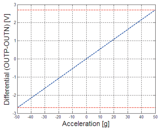
Figure 25: Differential acceleration output (OUTP-OUTN) at full scale
