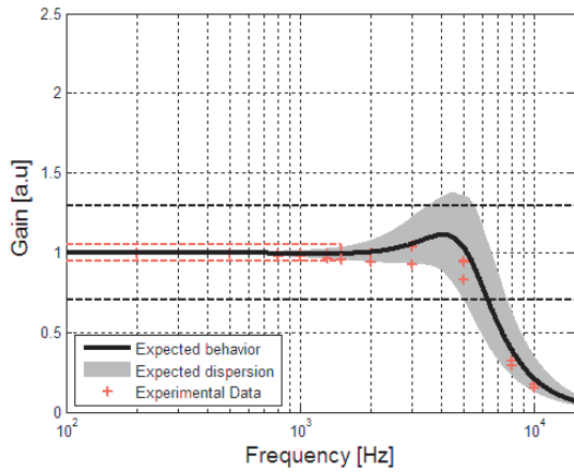
Figure 18: Typical high frequency response Courtesy of Customer
