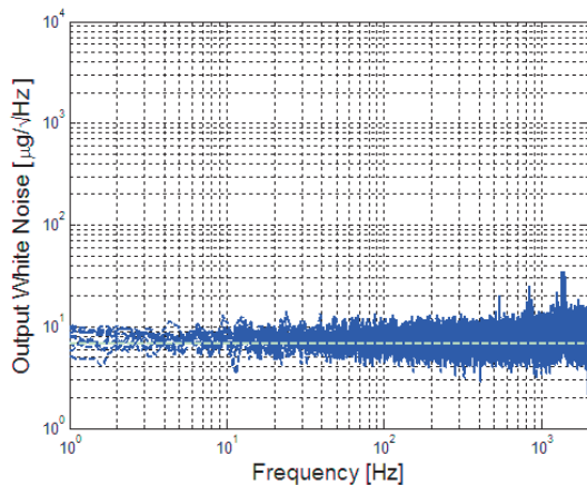
Figure 6: Typical white noise
