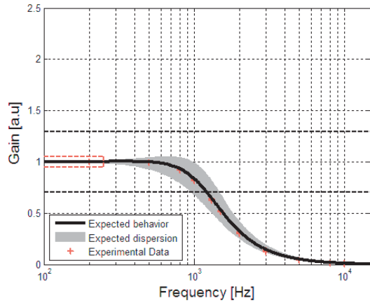
Figure 2: Typical high frequency response
