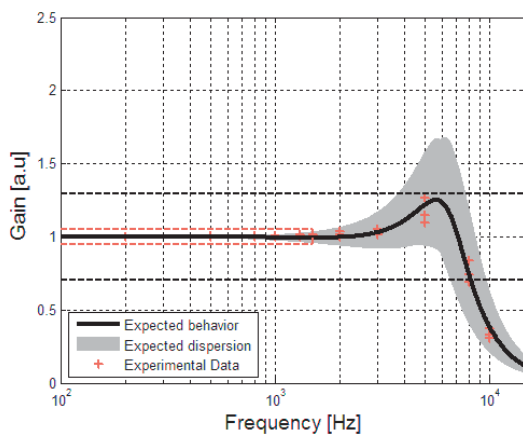
Figure 23: Typical high frequency response Courtesy of Customer
