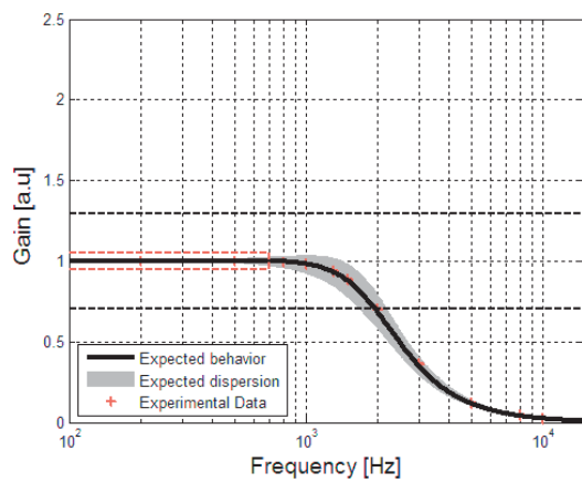
Figure 8: Typical high frequency response Courtesy of Customer
