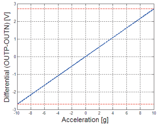
Figure 15: Differential acceleration output (OUTP-OUTN) at full scale
