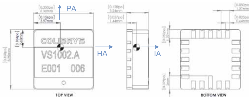
Figure 43: Package mechanical dimension
