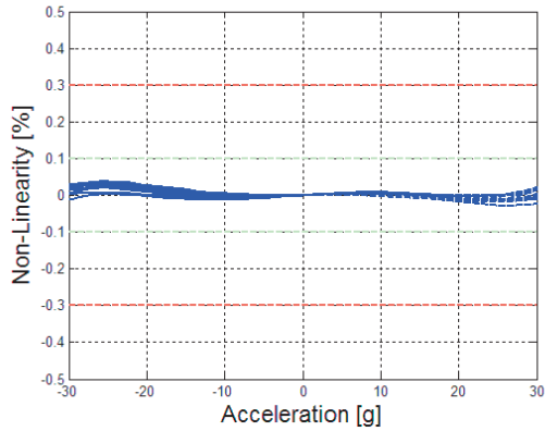
Figure 19 : Non linearity under vibration
