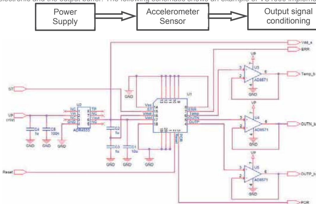
Figure 44: Recommended Block diagram & Schematic
