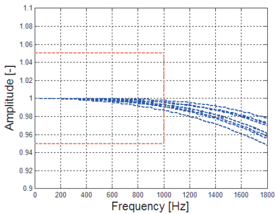
Figure 12: Typical frequency response in band
