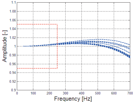
Figure 1: Typical frequency response in band
