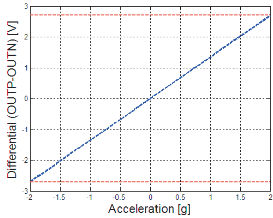
Figure 4: Differential acceleration output (OUTP-OUTN) at full scale
