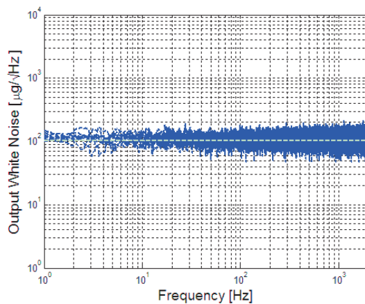
Figure 21: Typical white noise
