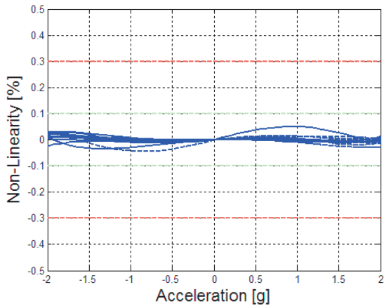
Figure 3 : Non linearity under vibration
