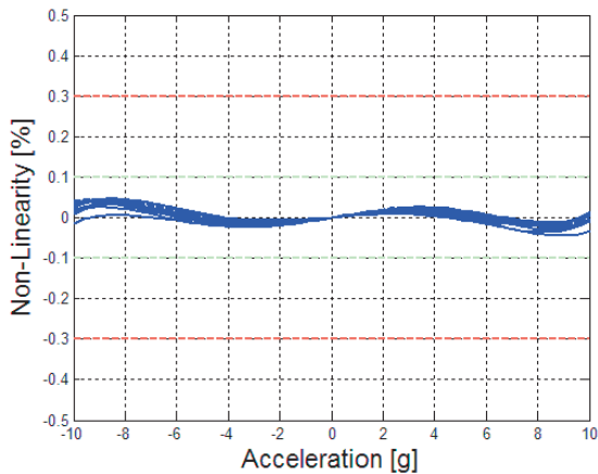
Figure 14 : Non linearity under vibration
