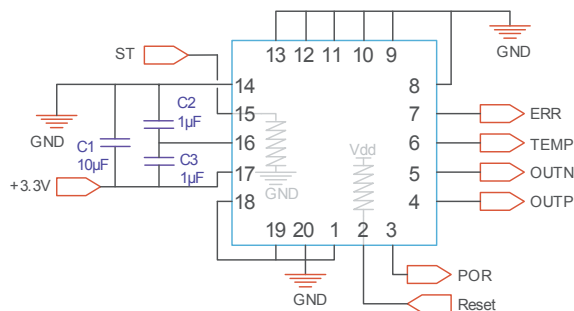
Figure 38: Proximity circuit & pull-up/down
