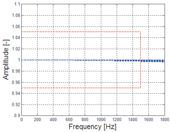
Figure 27: Typical frequency response in band
