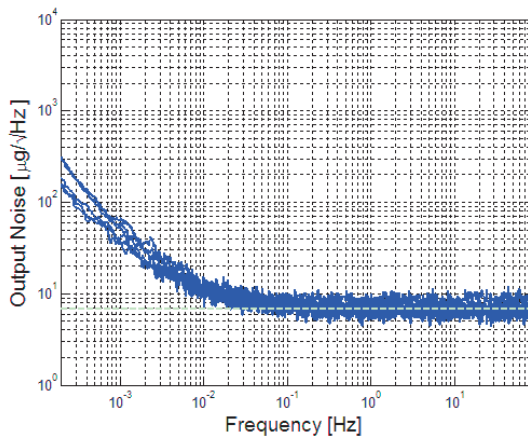
Figure 5: Typical Low Frequency Noise
