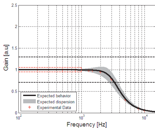
Figure 13: Typical high frequency response Courtesy of Customer
