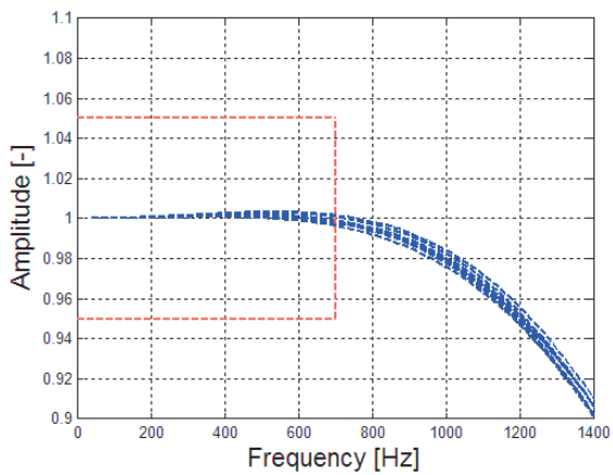
Figure 7: Typical frequency response in band
