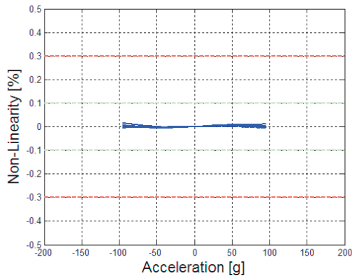
Figure 34 : Non linearity under vibration
