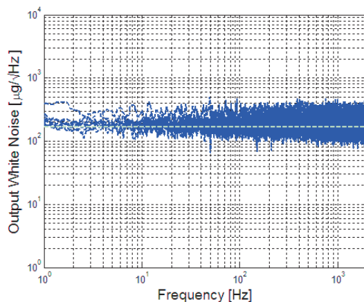
Figure 26: Typical white noise
