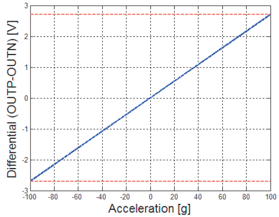
Figure 30: Differential acceleration output (OUTP-OUTN) at full scale
