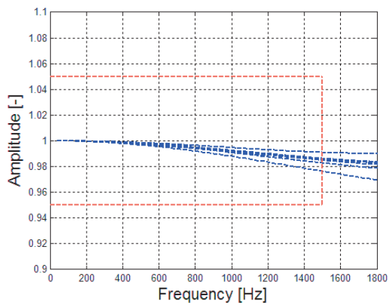
Figure 22: Typical frequency response in band
