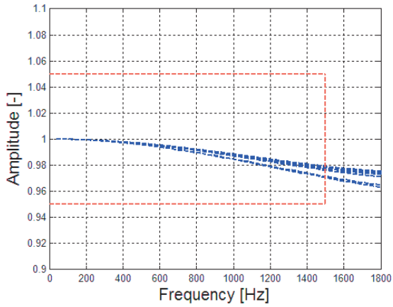
Figure 17: Typical frequency response in band
