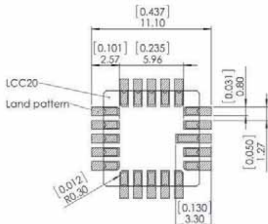
Figure 45 : LCC20 land pattern recommendation (unit are mm/[inch])
