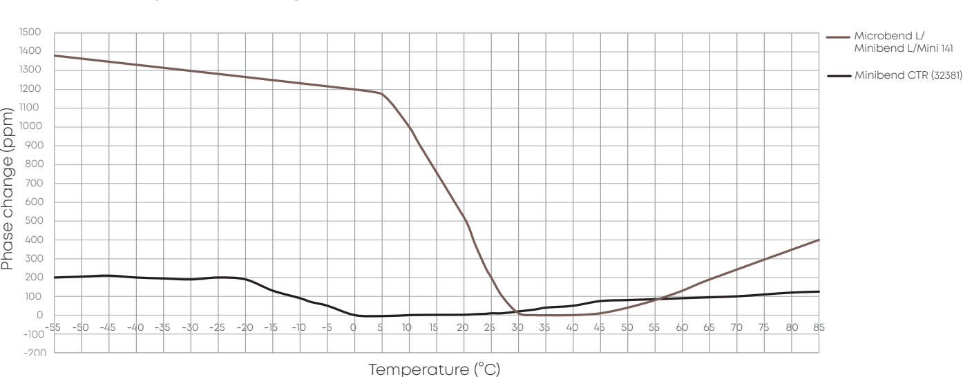
Phase stability versus temperature
