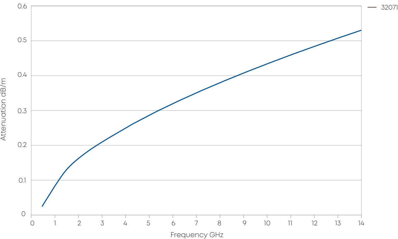
Attenuation (nominal values at +25 °C ambient temperature)
