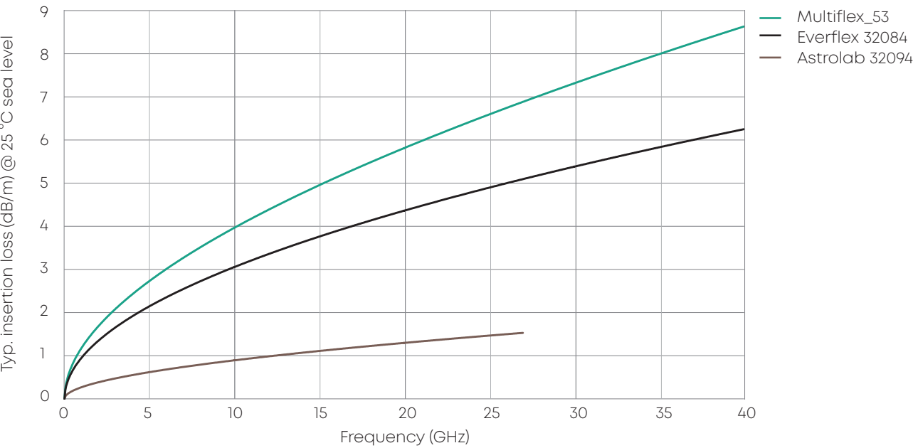
Attenuation (nominal values at +25 °C ambient temperature)
