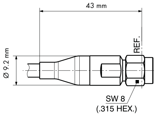
1.85 mm male (SF_11_PC185-501)
