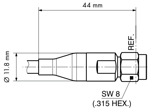
N male (SF_11_N-501)
