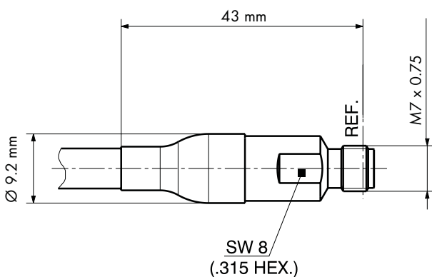
2.4 mm female (SF_21_PC24-501)
