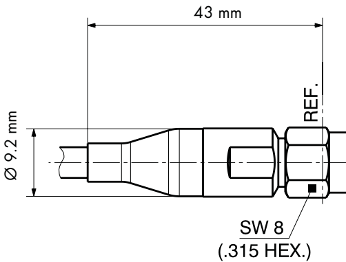
2.4 mm male (SF_11_PC24-501)
