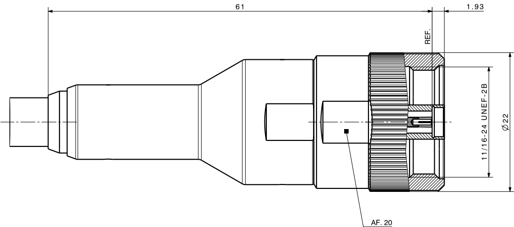
2.4 mm ruggedised PORT female (SF_21_PC24-502)
