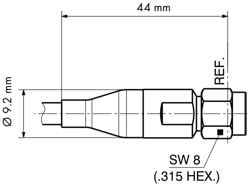
2.92 mm male (SF_11_SK-501)
