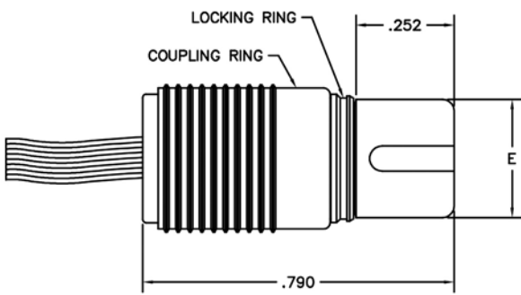
PLUG (Socket Contacts)
