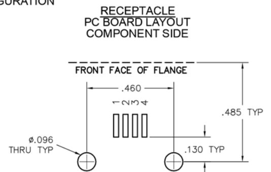
FOOTPRINT/PAD CONFIGURATION
