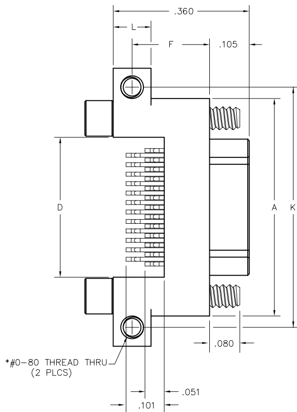
PLUG
