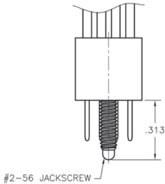
HARDWARE STYLE 61
